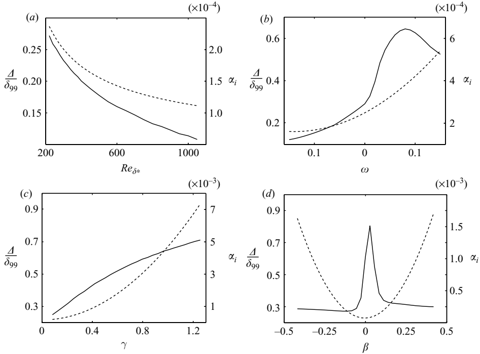
FIGURE 9. Penetration depth \Delta (—) and decay rate \alpha_i (---) of the continuous Orr–Sommerfeld modes for ranges of (a) Reynolds number Re_\delta , (b) angular frequency \omega , (c) wall-normal wavenumber \gamma and (d) spanwise wavenumber \beta . The plots are based on (Re_\delta, \omega; \beta, \gamma) = (220, -0.01; -0.14, 0.126) .
