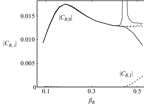
FIGURE 6. Thick lines: receptivity coefficients |C_{R,0}| (—) and |C_{R,1}| (---) according to (3.2). Thin lines: receptivity coefficient C_R , (3.1), as in figure 5(b).
