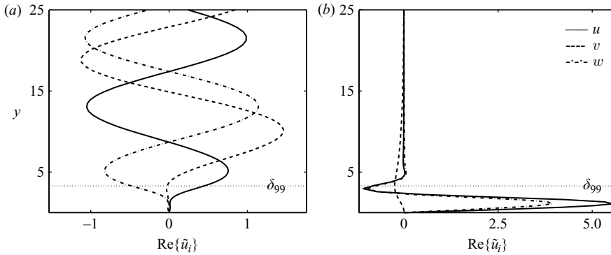
FIGURE 3. (a) Wall-normal shape of a free-stream eigenmode from the continuous spectrum of the Orr–Sommerfeld equation, (\alpha, \beta) = (0.130, -0.140) , \alpha_i = 0.00081 , \gamma = 0.377 , \omega = -0.01 . (b) Amplitude in the wall-normal direction of a travelling discrete boundary-layer eigenmode, (\alpha, \beta) = (0.102, -0.140) , \alpha_i = 0.00474 , \omega = -0.01 .
