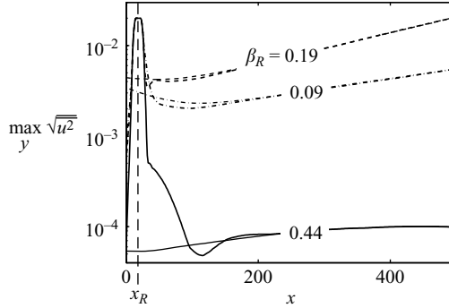
FIGURE 4. Boundary-layer response to roughness at x_R = 18.4 ( Re_{\delta^*} = 234 ), expressed as wall-normal maximum of the chordwise disturbance-velocity amplitude (thick lines), and evolution of the excited steady crossflow instability waves (thin lines).
