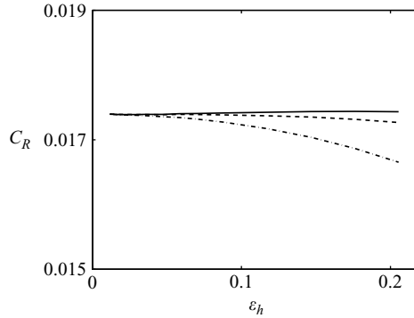
FIGURE 8. Effect of bump height on receptivity to surface roughness. \beta_R = 0.19 . Bump shape I (—), II (---) and III (-.-).
