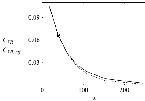
FIGURE 15. Coefficient for receptivity to free-stream vorticity combined with surface roughness versus chordwise location (—) and effective receptivity coefficient (---). The spanwise wavenumbers of the vortical mode and the roughness element are |\beta_V| = 0.381 and \beta_R = 0.190 (case (b) in figure 14). Circle: First neutral point of the excited unsteady crossflow wave.
