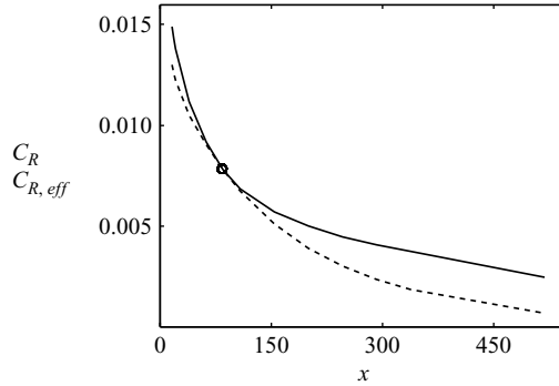
FIGURE 7. Receptivity coefficient for surface roughness as a function of the chordwise station x_R of the roughness element (—). Roughness shape III is used, and \beta_R = 0.126 . Effective receptivity coefficient C_{R,eff} (---). \circ , first neutral point of the excited steady cross-flow mode.
