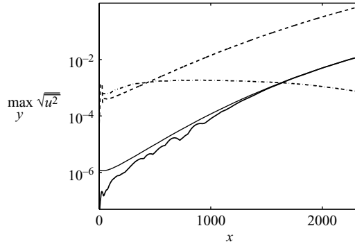
FIGURE 13. Combination of free-stream vorticity and surface roughness. The roughness element ( \beta_R = 0.190 ) excites an unstable steady eigenmode (---), while the vortical free-stream mode ( \beta_V = -0.381 ) does not trigger a growing travelling mode (---). In combination, however, they excite travelling crossflow instability (—, thick curve).
