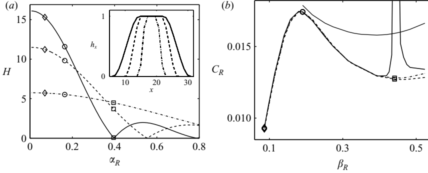
FIGURE 5. (a) Three roughness shapes in physical (inset) and spectral space. The symbols mark the Fourier component of the spectral bump shape at the chordwise wavenumber \alpha_{CF} of the excited steady crossflow eigenmode (i.e. \alpha_{CF} = \alpha_R ), shown for three spanwise wavenumbers of the roughness: \beta_R = 0.09 ( \diamond ), 0.19 ( \circ ) and 0.44 ( \square ). (b) Thick lines: receptivity coefficient in spatially evolving flow versus spanwise wavenumber of the roughness for the three bump shapes in (a). The roughness is placed at x_R = 18.4 ( Re_{\delta^*} = 234 ). The symbols correspond to those in (a). Thin solid line: receptivity coefficient in parallel flow.
