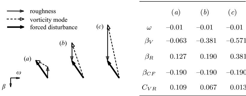
FIGURE 14. Interaction between a decaying unsteady disturbance due to free-stream vorticity and an amplifying steady disturbance caused by localized roughness. Three combinations of the spanwise wavenumbers \beta_V and \beta_R of the vortical mode and the roughness element are considered. Excitation of an unstable travelling crossflow mode with spanwise scale \beta_{CF} = -0.190 .
