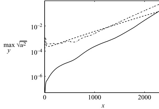
FIGURE 16. Combination of free-stream vorticity and surface roughness. Both the roughness element ( \beta_R = 0.095 , ---) and the vortical free-stream mode ( \beta_V = -0.095 , -·-) excite unstable crossflow eigenmodes, which interact and force a harmonic wave with \beta_f = -0.190 (—).
