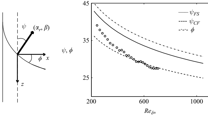
FIGURE 10. Horizontal wavenumber angle \psi = \arctan(\alpha_r/|\beta|) for the continuous Orr–Sommerfeld mode ( \omega = -0.01 , \beta = -0.14 , \gamma = 0.126 , —) and the excited travelling crossflow wave (---) and local angle \phi of the external streamline (-.-). The symbols mark the wave angle of the forced boundary-layer disturbance and are extracted from DNS data.
