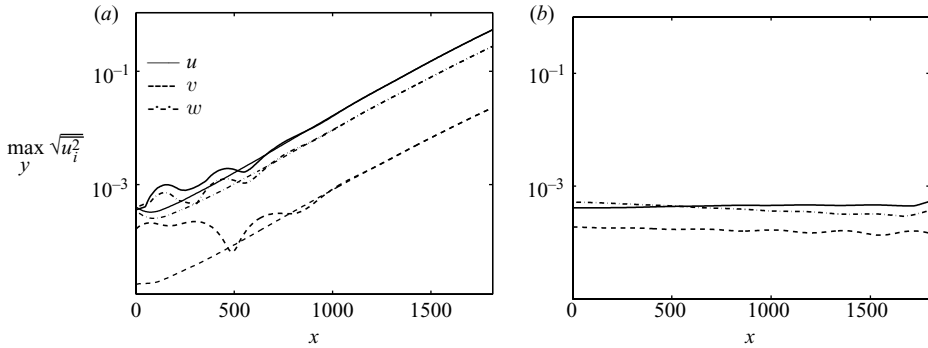
FIGURE 11. (a) Response of the non-parallel three-dimensional boundary layer to free-stream vorticity. Thick lines: spatial evolution of the boundary-layer disturbance, excited by a continuous Orr–Sommerfeld mode ( \omega = -0.01 , \beta = -0.14 , \gamma = 0.126 ) at Re_{\delta^*} = 220 . Thin lines: spatial evolution of the corresponding crossflow instability wave. (b) Response of a parallel Falkner–Skan–Cooke boundary layer at Re_{\delta^*} = 360 to a continuous Orr–Sommerfeld mode ( \omega = -0.01 , \beta = -0.14 , \gamma = 0.126 ).
