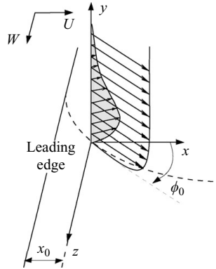
FIGURE 1. Wall-normal profiles of the streamwise and the crossflow velocity for Falkner-Skan-Cooke boundary-layer flow.
