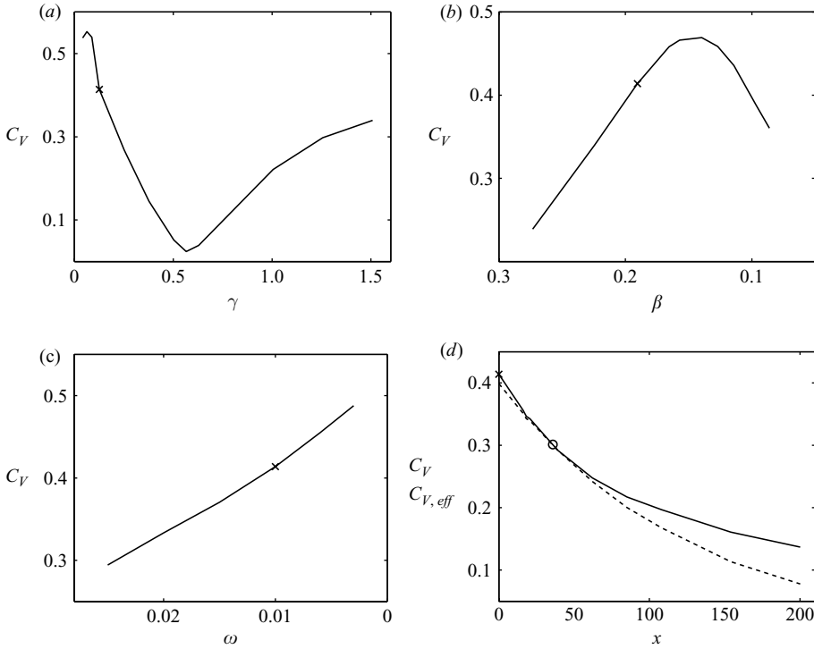
FIGURE 12. Dependence of the receptivity coefficient to free-stream vorticity on (a) the wall-normal wavenumber, (b) the spanwise wavenumber and (c) the angular frequency of the vortical mode. In (d), the influence of the chordwise station on C_V is shown, at which the free-stream disturbance is prescribed (—). Effective receptivity coefficient (---). \circ , the first neutral point of the excited unsteady crossflow mode. The plots are based on (Re_{\delta^*}, \omega; \beta, \gamma) = (220, -0.01; -0.19, 0.126) , marked by the cross.
