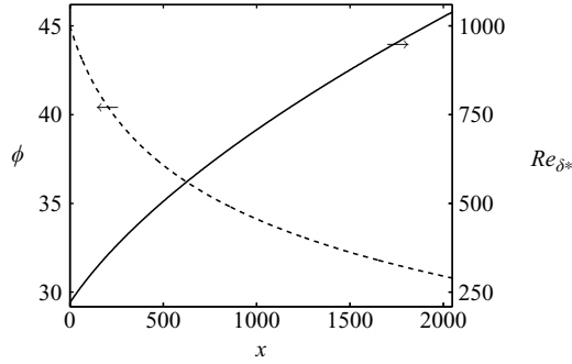
FIGURE 2. Reynolds number (—) and external streamline angle (---) as a function of the chordwise coordinate.
