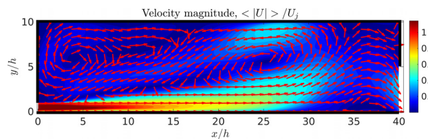
Fig. 6 Temporal and spatial (in spanwise direction) averaged velocity magnitude contour with velocity vectors
