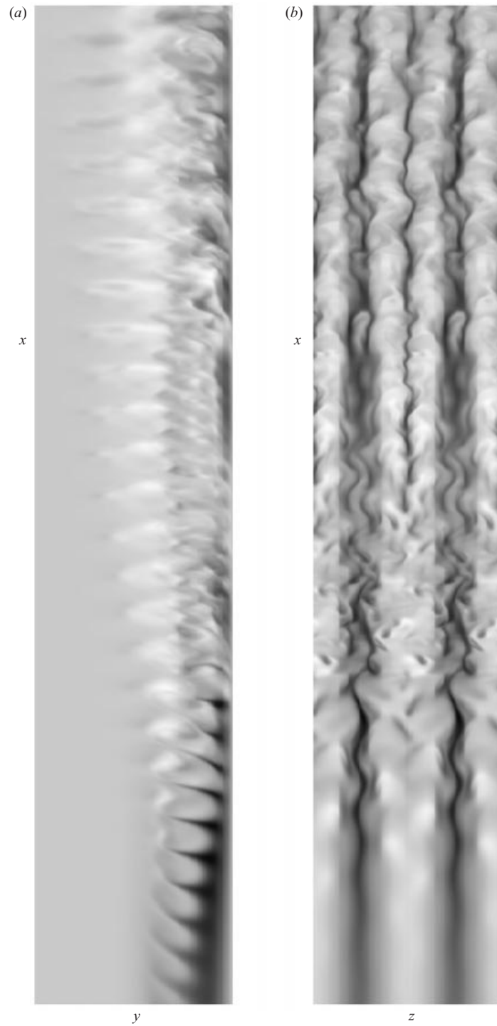
FIGURE 17. Visualization of streak breakdown using the streamwise velocity component of the perturbation in (a) a wall-normal (x, y) -plane at z = 0 and (b) a wall-parallel (x, z) -plane at y = 0.45 . x \in [185, 360] . Grey scale from dark to light corresponds to negative to positive values. The flow is from bottom to top. In (b) two spanwise streaks are displayed.
