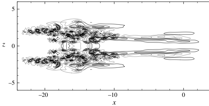
FIGURE 17. Turbulent spot in contours of v' at t = 40 and y = -0.56 during the evolution of a large vortex pair ( \epsilon = 0.2097 ) in Newtonian flow. Contour spacing 3.75 \times 10^{-2} .
