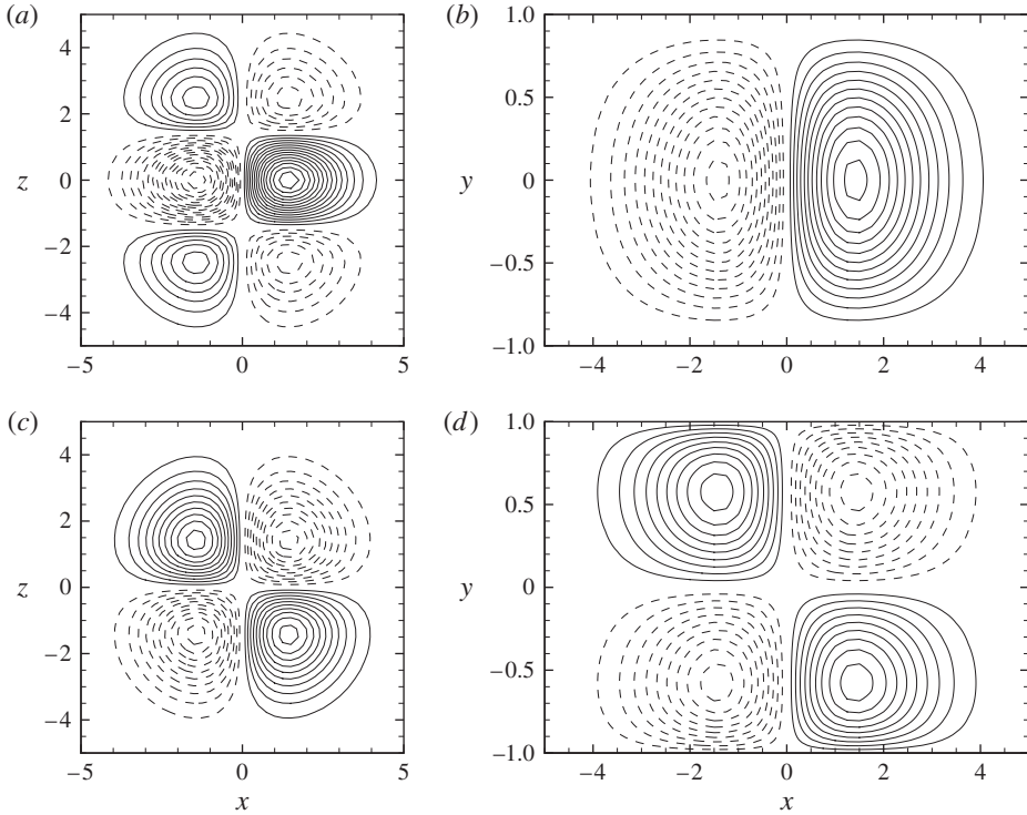
FIGURE 3. Initial wall-normal and spanwise velocity perturbation fields: (a) v' at y = -0.56 , contour spacing 2.0 \times 10^{-6} ; (b) v' at z = -1.0 , contour spacing 2.0 \times 10^{-6} ; (c) w' at y = -0.56 , contour spacing 8.0 \times 10^{-6} ; (d) w' at z = -1.0 , contour spacing 8.0 \times 10^{-6} . Solid and dashed lines indicate positive and negative velocities, respectively.
