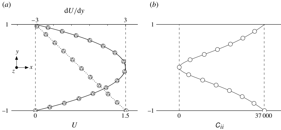
FIGURE 2. Mean velocity profile, mean shear, and trace of the conformation tensor at t = 0 for Re = 2000 : \dots , dU/dy ; \Delta , Newtonian flow; \circ , non-Newtonian flow at We = 100 , L_{max} = 300 and \beta = 0.9 .
