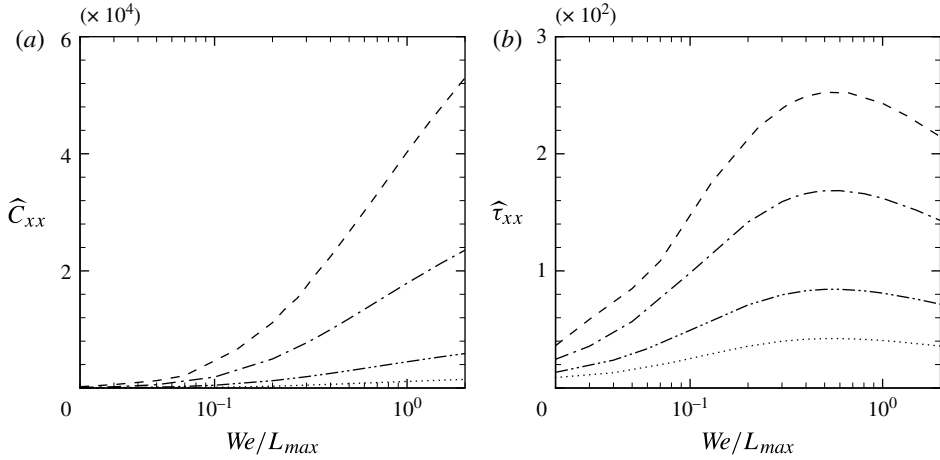
FIGURE 13. Variation of 'xx' component of the mean conformation tensor and polymeric stress tensor: \cdots , L_{max} = 50 ; -\cdot-\cdot- , L_{max} = 100 ; -\cdot-\cdot- , L_{max} = 200 ; - - - , L_{max} = 300 .
