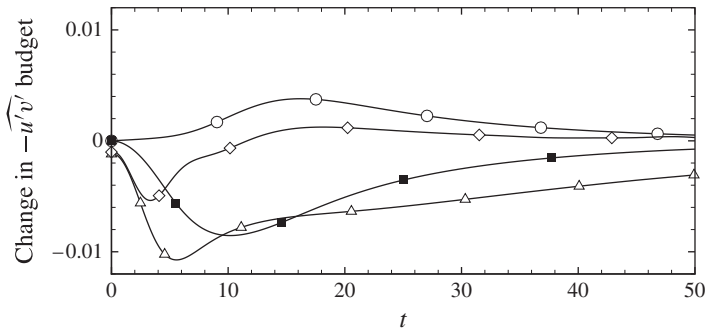
FIGURE 10. Difference between the corresponding components of the shear stress budget in non-Newtonian and Newtonian flow: \Delta , [-\widehat{\mathcal{P}}_{xy}/2E_0] ; \circ , [-\widehat{\mathcal{C}}_{xy}/2E_0] ; \blacksquare , -\widehat{\mathcal{W}}_{xy}/2E_0 ; \diamond , [-(1/2E_0)\partial \widehat{u'v'}/\partial t] .
