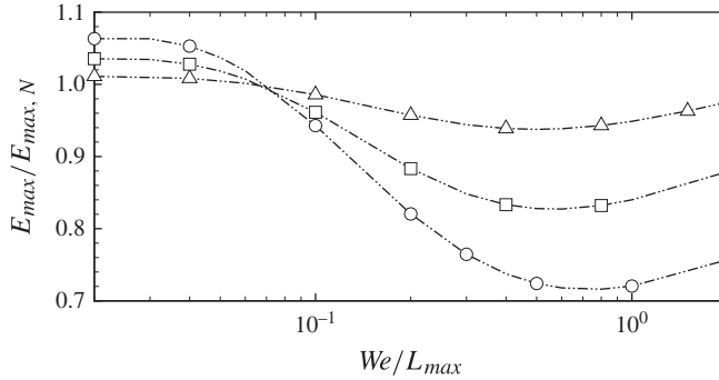
FIGURE 14. The effect of polymer concentration, represented by \beta , on the maximum perturbation energy in non-Newtonian flow: \Delta , \beta = 0.9 ; \square , \beta = 0.7 ; \circ , \beta = 0.5 .
