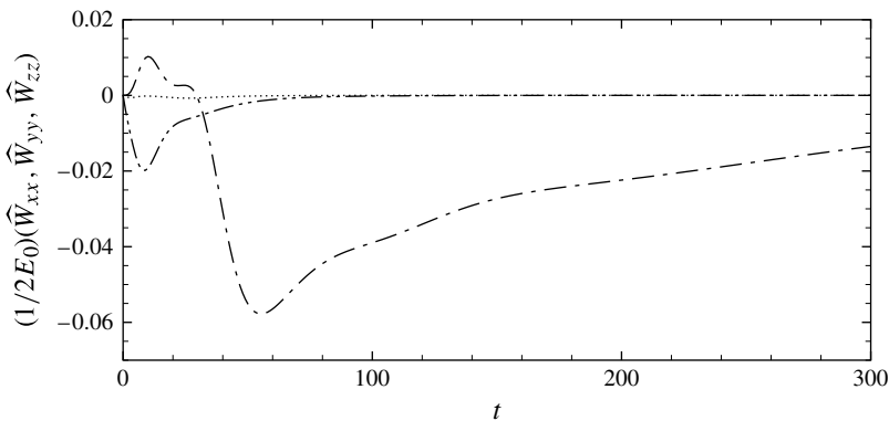
FIGURE 19. Evolution of the components of polymer work for \epsilon = 0.10485 , We = 15 , L_{max} = 100 and \beta = 0.9 : — · —, \widehat{W}_{xx} ; ····, \widehat{W}_{yy} ; — · · —, \widehat{W}_{zz} .
