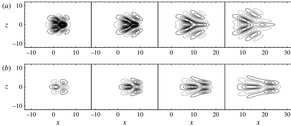
FIGURE 4. Evolution of the disturbance ( \epsilon = 1.5 \times 10^{-4} ) in Newtonian flow at y = -0.56 and t = \{3, 7, 13, 20\} . Contours denote (a) wall-normal v' and (b) streamwise u' velocity perturbations.
