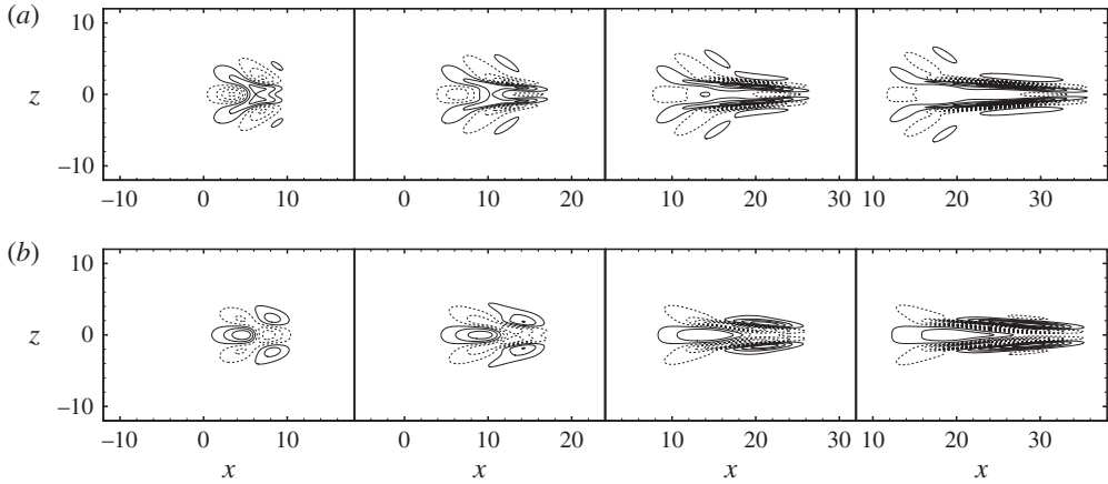
FIGURE 16. Evolution of the disturbance ( \epsilon = 0.10485 ) in Newtonian flow at y = -0.56 and t = [7, 13, 20, 27] ; (a) wall-normal v' and (b) streamwise u' velocity perturbations.
