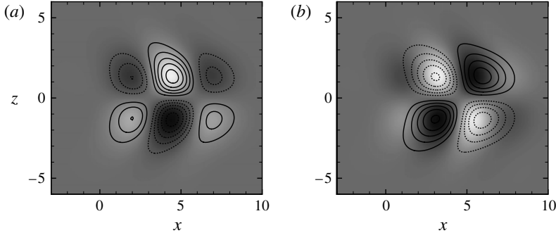
FIGURE 9. Snapshots at t = 4 , y = -0.56 during the evolution of the small-amplitude vortex pair in non-Newtonian flow at We = 40 , L_{max} = 300 and \beta = 0.9 . (a) Contour lines, \partial w'/\partial x (contour spacing 2 \times 10^{-5} ); flood, c'_{xz} (contour range [-3, 3] ). (b) Contour lines, w' (contour spacing 2 \times 10^{-5} ); flood, \partial \tau'_{xz}/\partial x (contour range [-8 \times 10^{-2}, 8 \times 10^{-2}] ).
