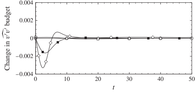
FIGURE 11. Difference between the corresponding components of \partial \overline{v'^2} / \partial t (see (3.2)) in non-Newtonian and Newtonian flow: \Delta , [\widehat{\mathcal{P}}_{yy} / 2E_0] ; \circ , [\widehat{\epsilon}_{yy} / 2E_0] ; \blacksquare , \widehat{\mathcal{W}}_{yy} / 2E_0 ; \diamond , [(1/2E_0)\partial \overline{v'v'} / \partial t] .
