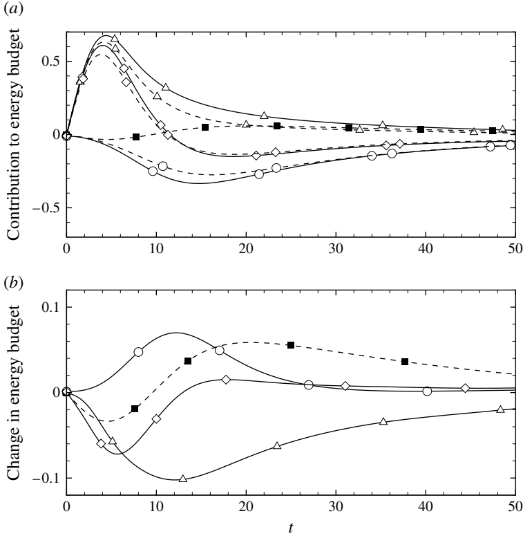
FIGURE 7. Components of the perturbation energy budget (see (3.3)): (a) —, Newtonian flow; ----, non-Newtonian flow at L_{max} = 300 , \beta = 0.9 , We = 40 ; \Delta , \widehat{\mathcal{P}}_{ii}/2E_0 ; \circ , \widehat{\epsilon}_{ii}/2E_0 ; \blacksquare , \widehat{\mathcal{W}}_{ii}/2E_0 ; \diamond , (1/2E_0)\partial\widehat{u}'_i\widehat{u}'_i/\partial t ; (b) \Delta , [\widehat{\mathcal{P}}_{ii}/2E_0] ; \circ , [\widehat{\epsilon}_{ii}/2E_0] ; \blacksquare , [\widehat{\mathcal{W}}_{ii}/2E_0] ; \diamond , [(1/2E_0)\partial\widehat{u}'_i\widehat{u}'_i/\partial t] .
