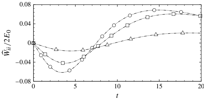
FIGURE 15. The effect of \beta on polymer work during the evolution of the small amplitude vortex pair at We = 30 and L_{max} = 100 : \Delta , \beta = 0.9 ; \square , \beta = 0.7 ; \circ , \beta = 0.5 .
