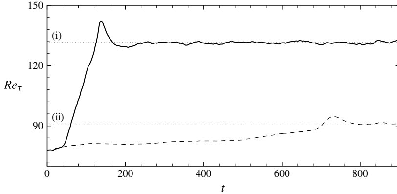
FIGURE 22. Effect of the addition of polymers to the process of transition: —, Newtonian; ----, non-Newtonian at We = 15 , L_{max} = 100 and \beta = 0.9 . The dotted lines mark Re_\tau in fully turbulent flow for the Newtonian (i) and non-Newtonian (ii) cases.
