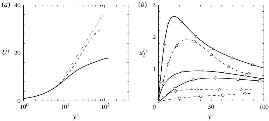
FIGURE 24. Statistics from fully turbulent flow: —, Newtonian; - - -, non-Newtonian at We = 15 , L_{max} = 100 and \beta = 0.9 ; (a) mean velocity profiles; \cdots , Virk asymptote for MDR; (b) root-mean-squared velocity fluctuations; \Delta , streamwise; \diamond , spanwise; \circ , wall-normal.
