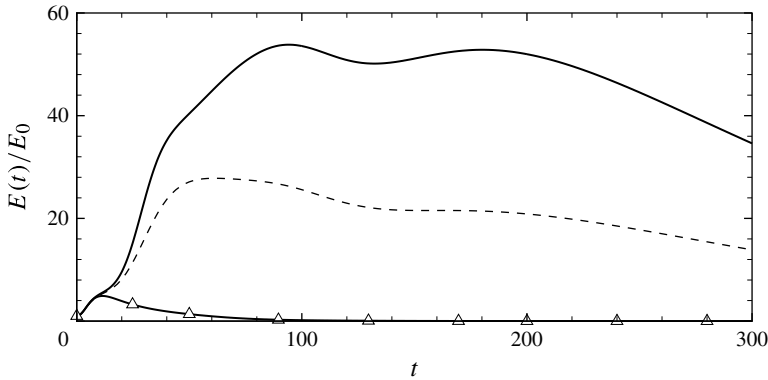
FIGURE 18. Evolution of energy amplification for \epsilon = 0.10485 : —, Newtonian flow; ----, non-Newtonian flow at L_{max} = 100 , \beta = 0.9 and We = 15 ; \Delta , \epsilon = 0.00015 .
