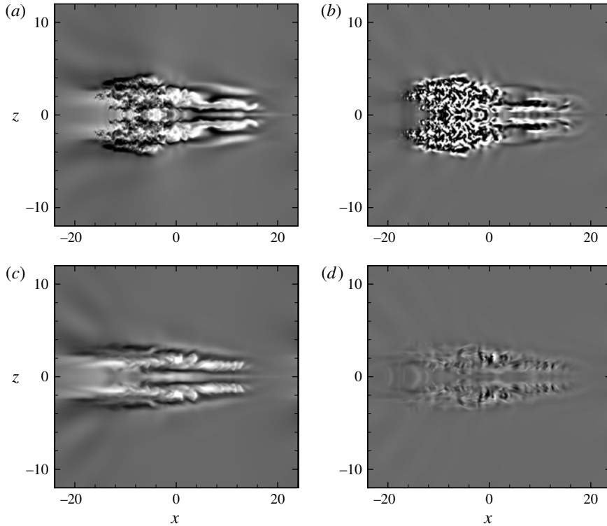
FIGURE 21. Snapshots of perturbation velocity at t = 50 and y = -0.56 during the evolution of the large-amplitude vortex pair. Newtonian flow: (a) u' = [-0.3, 0.3] ; (b) v' = [-0.05, 0.05] . Non-Newtonian flow at We = 15 , L_{max} = 100 and \beta = 0.9 : (c) u' ; (d) v' with the same contour limits.
