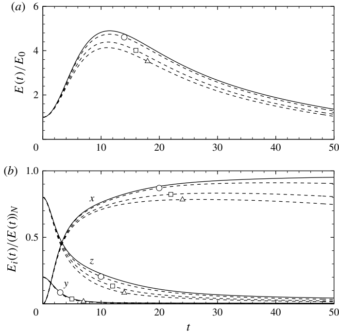
FIGURE 5. Evolution of perturbation energy for \epsilon = 1.5 \times 10^{-4} . (a) Amplification of total perturbation energy normalized by the initial value. (b) Components of perturbation energy, E_i(t) , normalized by the total energy in the Newtonian flow, (E(t))_N . —, Newtonian flow; ----, non-Newtonian flow at L_{max} = 300 and \beta = 0.9 ; \circ , We = 15 ; \square , We = 40 ; \triangle , We = 100 .
