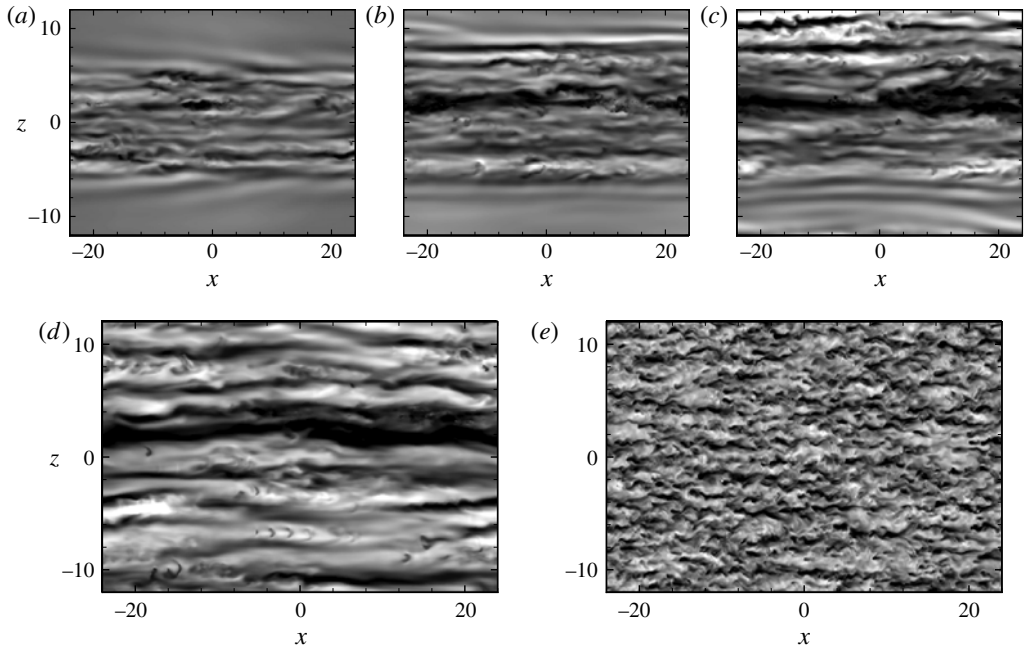
FIGURE 23. Snapshots of u' at y = -0.56 during the evolution of the large-amplitude vortex pair: (a–c) non-Newtonian flow during transition at We = 15 , L_{max} = 100 , \beta = 0.9 and t = \{200, 400, 600\} ; (d) and (e) are a comparison of non-Newtonian and Newtonian flows, respectively, at t = 900 . Contour limits: [-0.2, 0.2] .
