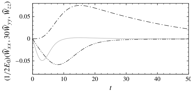
FIGURE 8. Evolution of the components of polymer work for We = 40 , L_{max} = 300 and \beta = 0.9 ; -\cdot-\cdot- , \widehat{\mathcal{W}}_{xx}/2E_0 ; \cdots\cdots , 30\widehat{\mathcal{W}}_{yy}/2E_0 ; -\cdot\cdot- , \widehat{\mathcal{W}}_{zz}/2E_0 .
