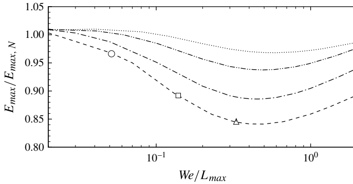
FIGURE 6. The effect of elasticity on the maximum perturbation energy in non-Newtonian flow: \cdots , L_{max} = 50 ; -\cdot-\cdot- , L_{max} = 100 ; -\cdot-\cdot- , L_{max} = 200 ; - - - - , L_{max} = 300 ; \circ , We = 15 ; \square , We = 40 ; \triangle , We = 100 .
