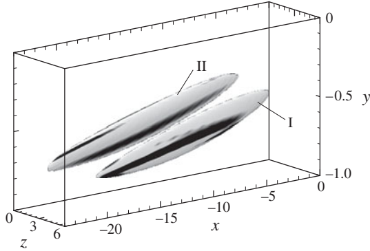
FIGURE 20. Isosurfaces of the streamwise perturbation velocity (I, u' = 0.2 ; and II, u' = -0.2 ), coloured by the streamwise polymer work at t = 40 . Contour levels range from \mathcal{W}_{xx}/2E_0 = -3.3 (black) to \mathcal{W}_{xx}/2E_0 = -1.1 (white).
