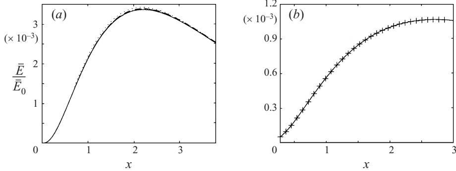
FIGURE 7. The spatial energy growth versus the streamwise coordinate, for the spanwise wavenumber, \beta = 0.45 . (a) With three small-amplitude solutions to the Navier–Stokes equations for Reynolds numbers (– – –, Re = 1 \times 10^6 ; – · – ·, Re = 5 \times 10^5 ; · · · ·, Re = 1 \times 10^5 ), and (—) one Reynolds number independent solution from the linearized, steady boundary layer approximations. (b) With an initial amplitude large enough to induce considerable nonlinear effects, A = 0.30 . Here the two curves represent solutions to the Navier–Stokes equations for two different Reynolds numbers (—, Re = 5 \times 10^5 ; +, Re = 7.5 \times 10^5 ).
